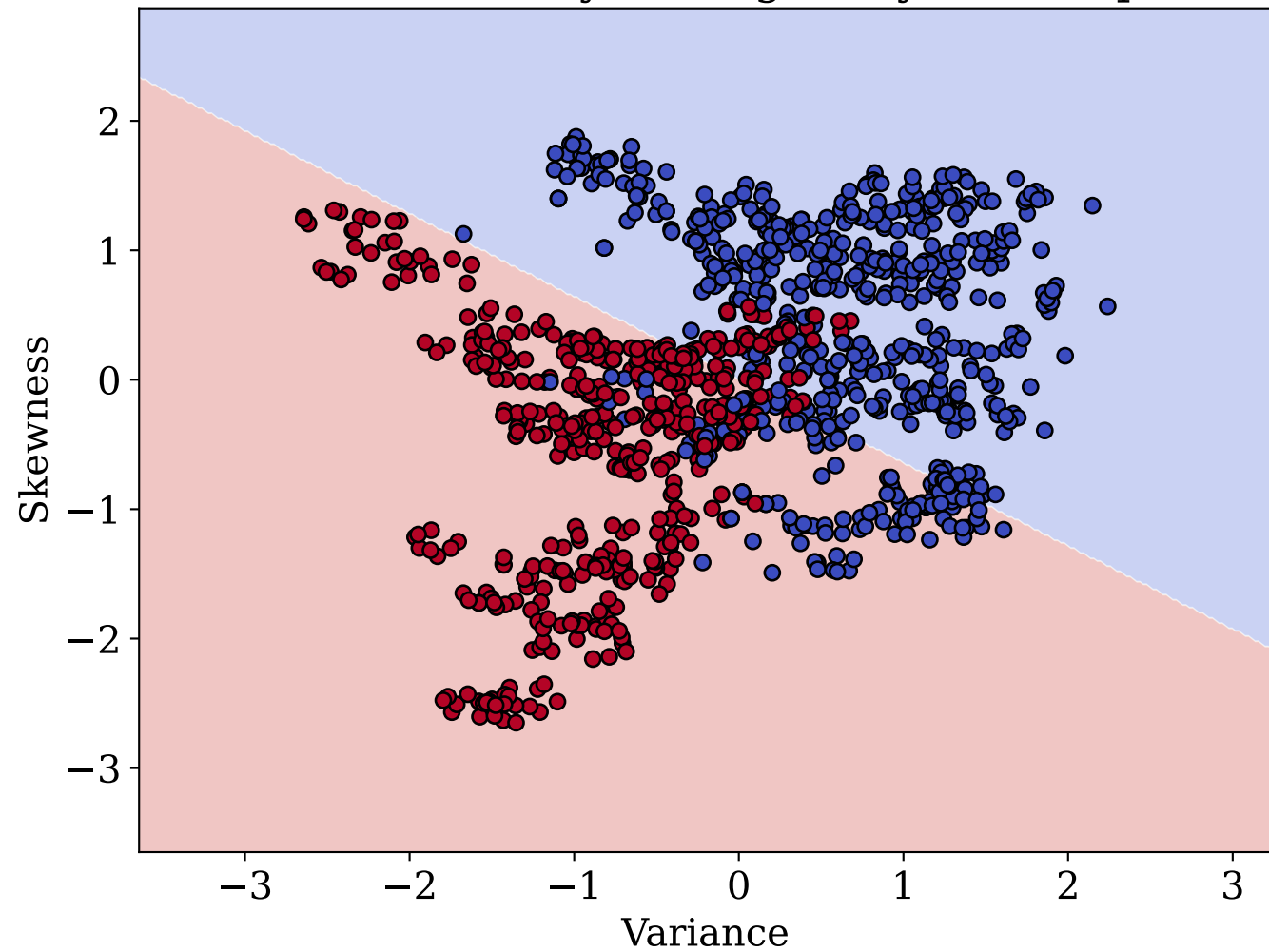
Decision Boundary of Single Layer Perceptron
